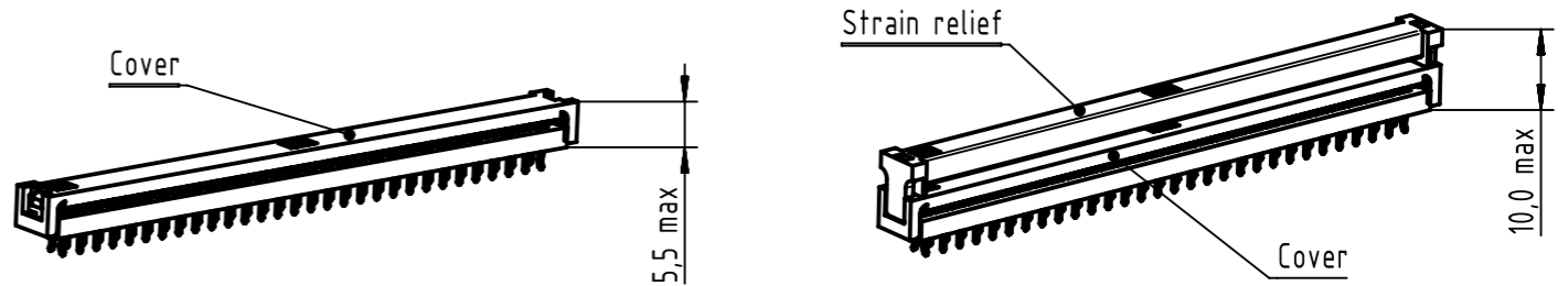
Assembled cover without strain relief
